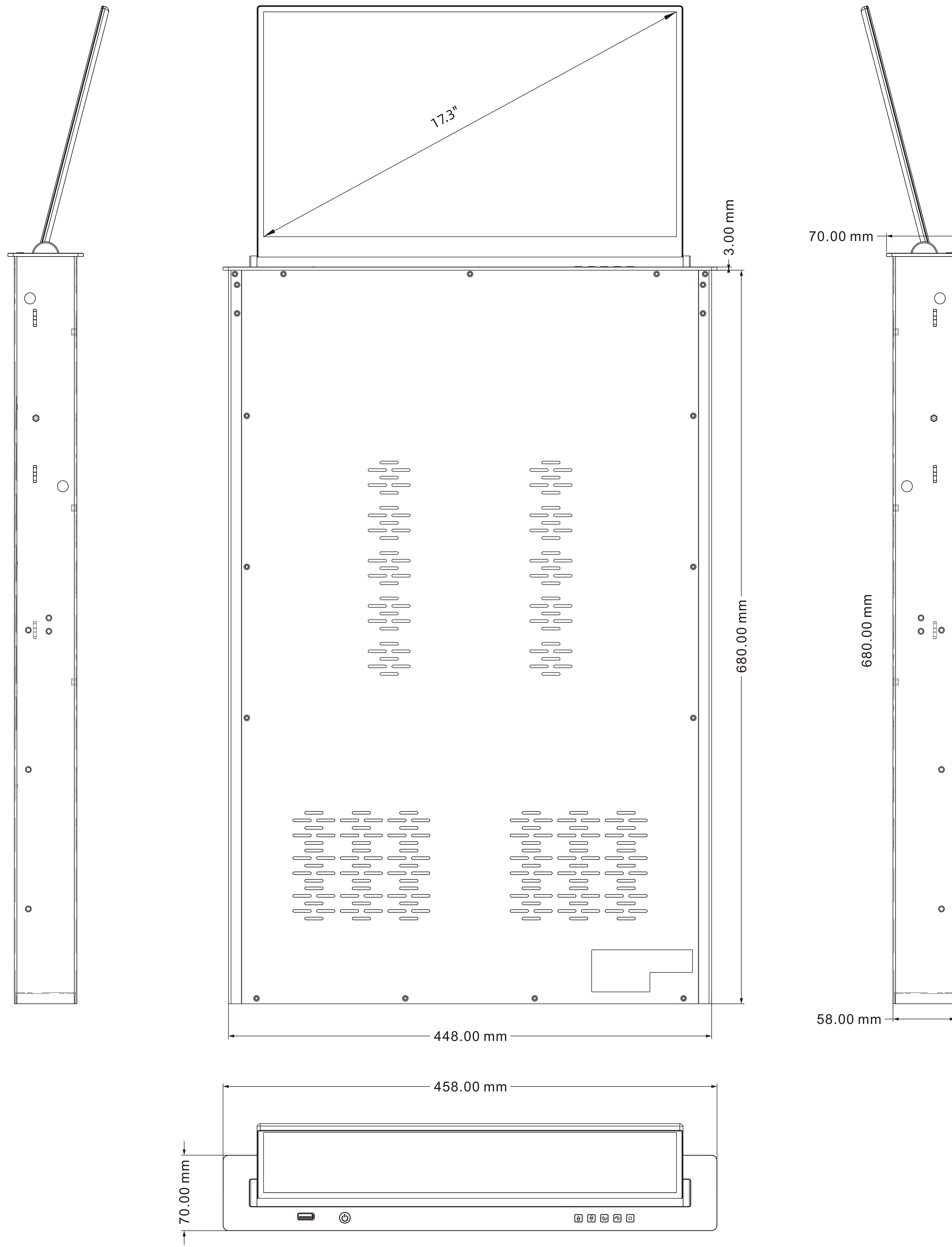
VIS-17LSSC-A Size(mm): 458(L)x70(W)x680(H)
