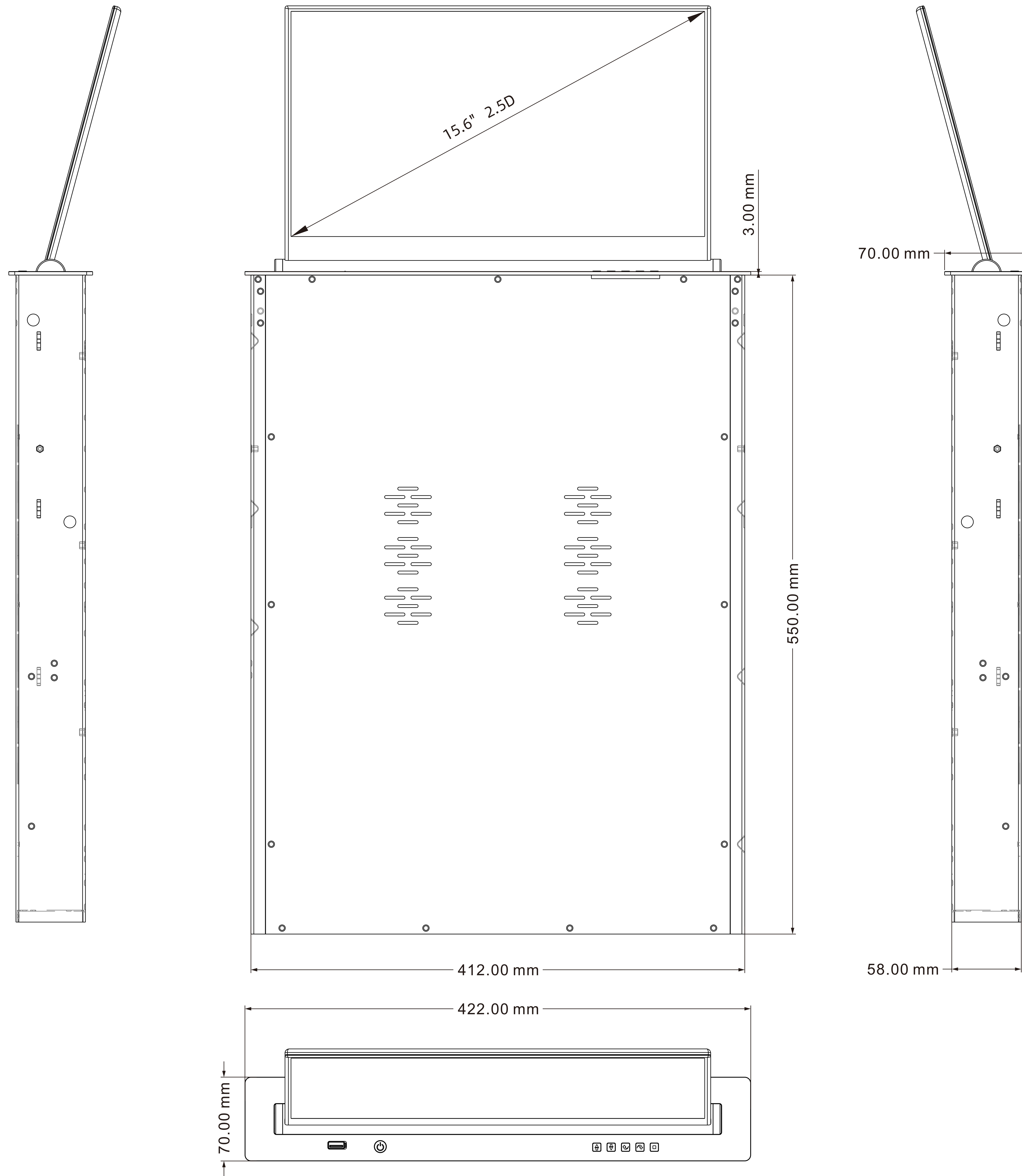
VIS-15LSSC Size(mm): 422(L)x70(W)x550(H)
