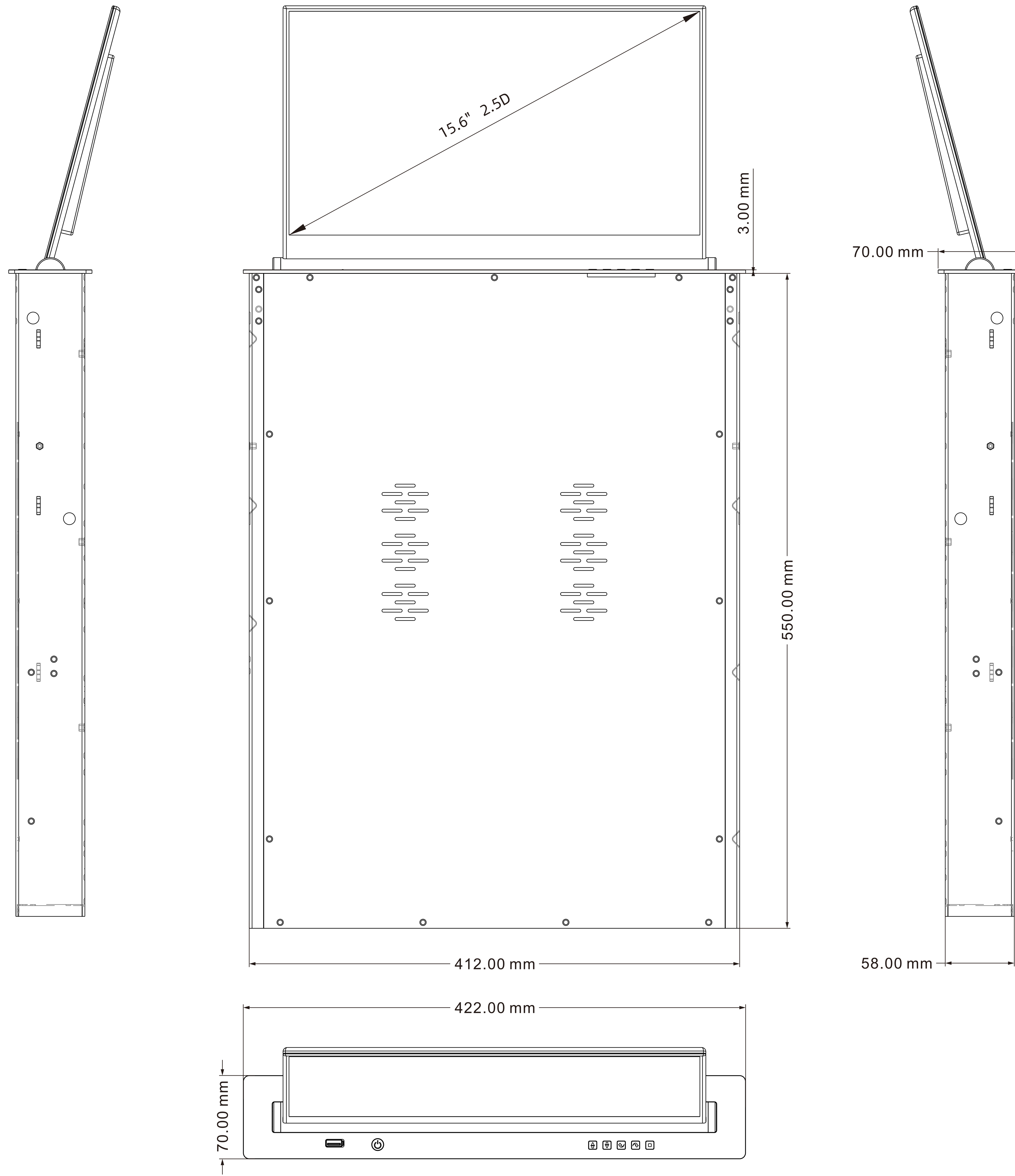
VIS-15LDSC Size(mm): 422(L)x70(W)x550(H)
