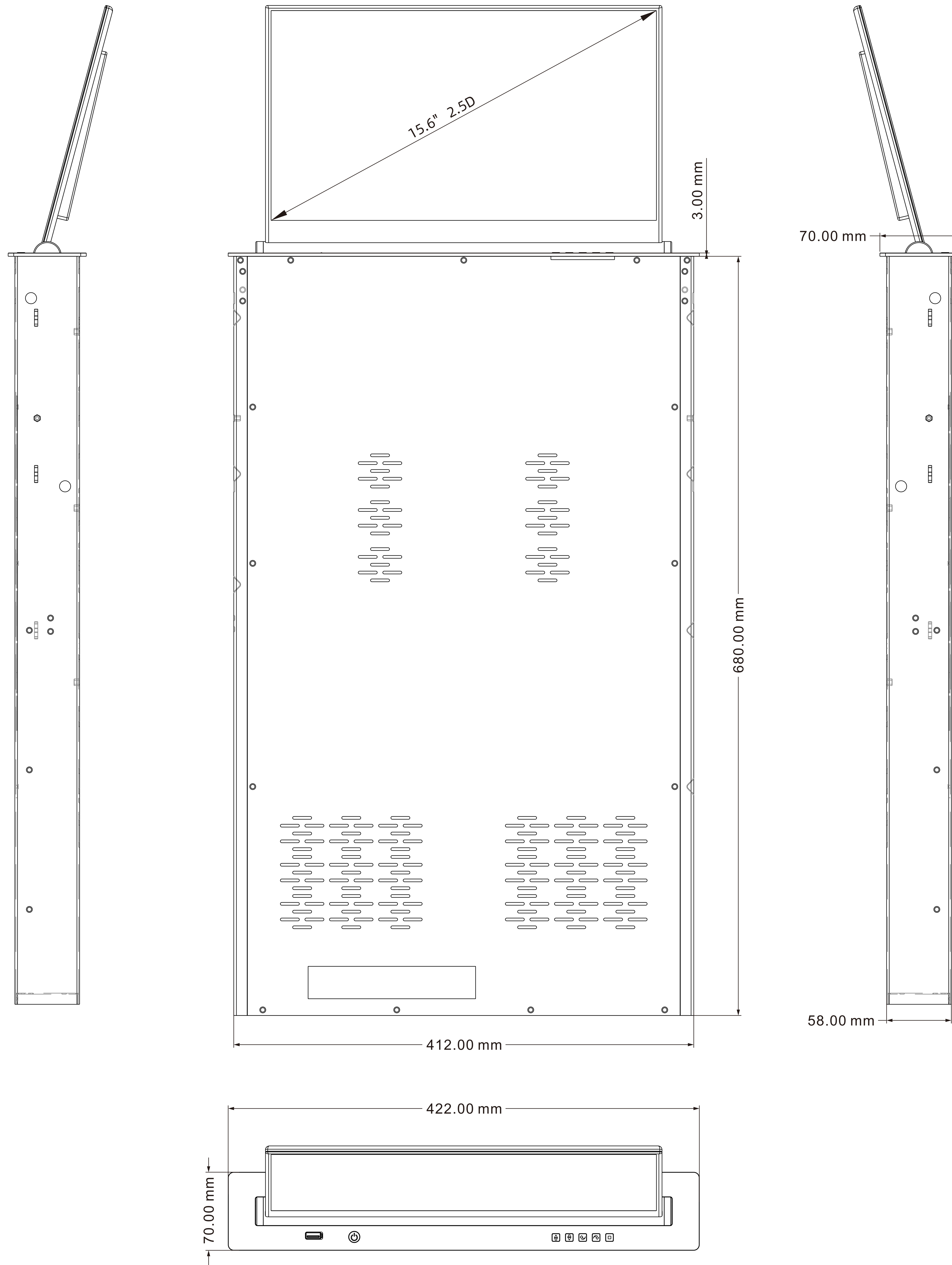
VIS-15LDSC-A Size(mm): 422(L)x70(W)x680(H)
